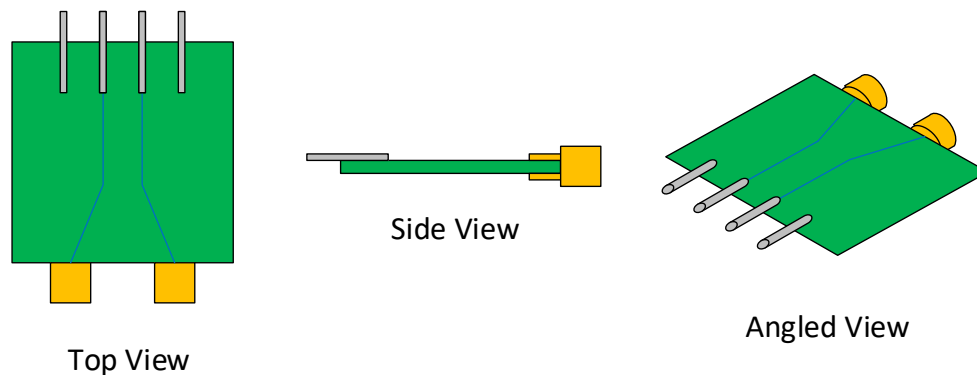
Figure A. 1: 2-pin to SMA Adapter 1
