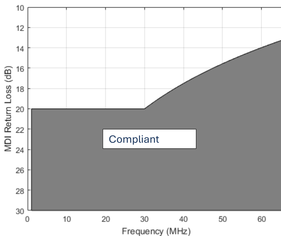
Figure 2: MDI return loss
