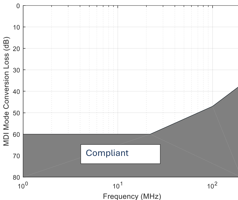
Figure 3: MDI mode conversion loss
