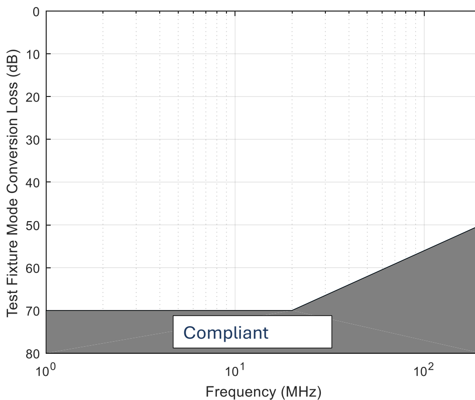
Figure 4: Test fixture mode conversion loss
