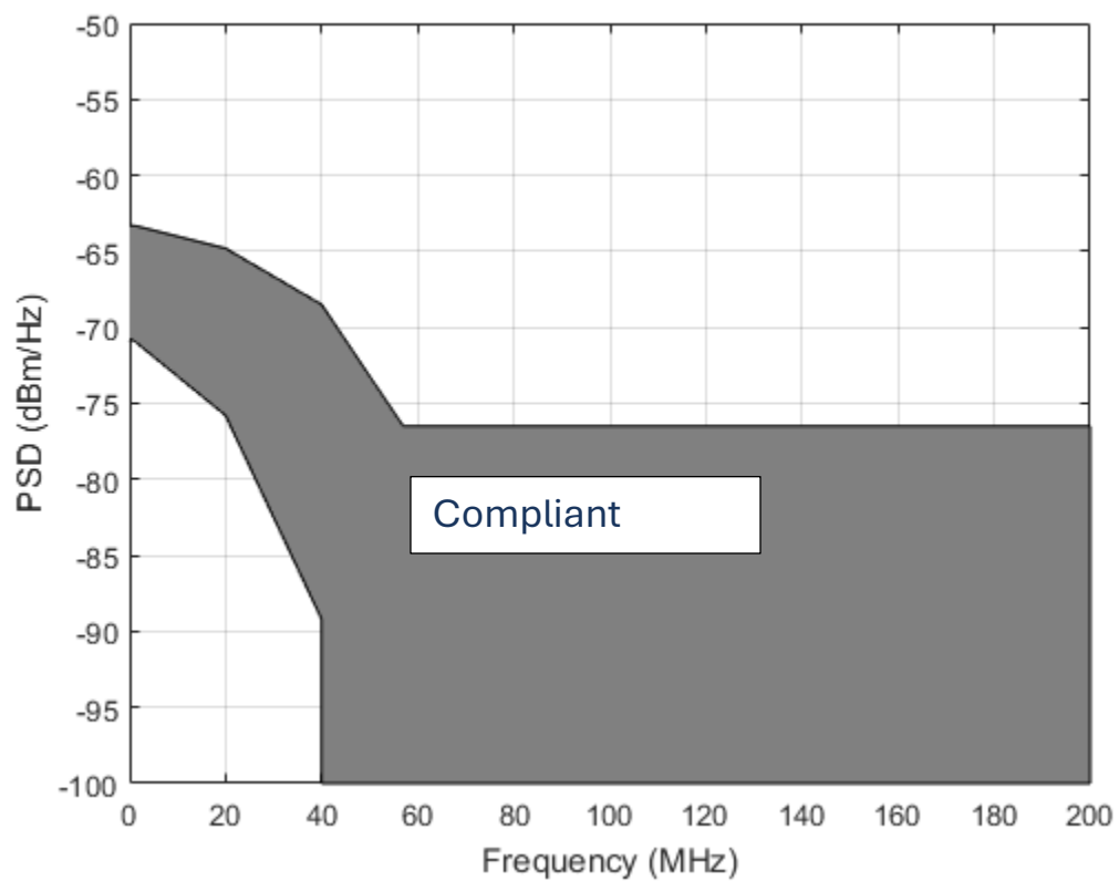
Figure 1: Transmitter PSD mask
