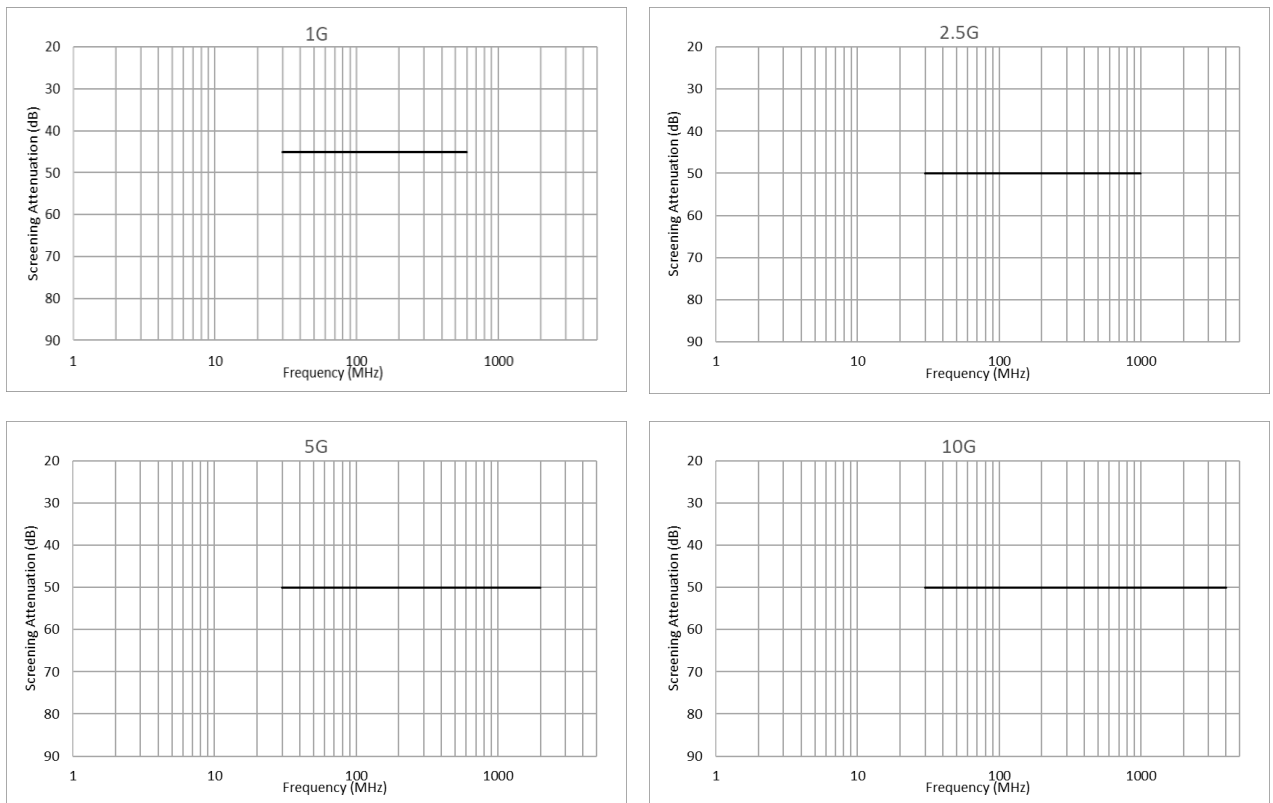
Figure 71: Screening attenuation requirements for connectors
