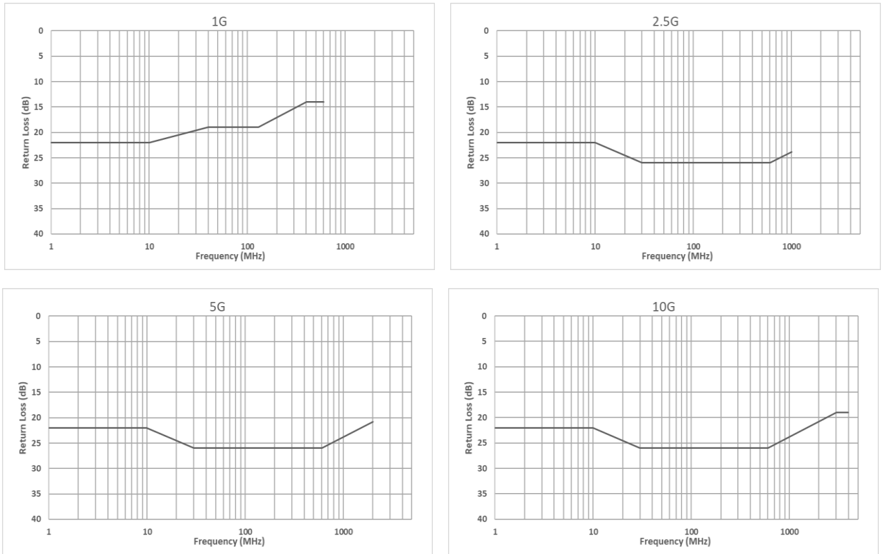
Figure 63:Return loss limit for cables
