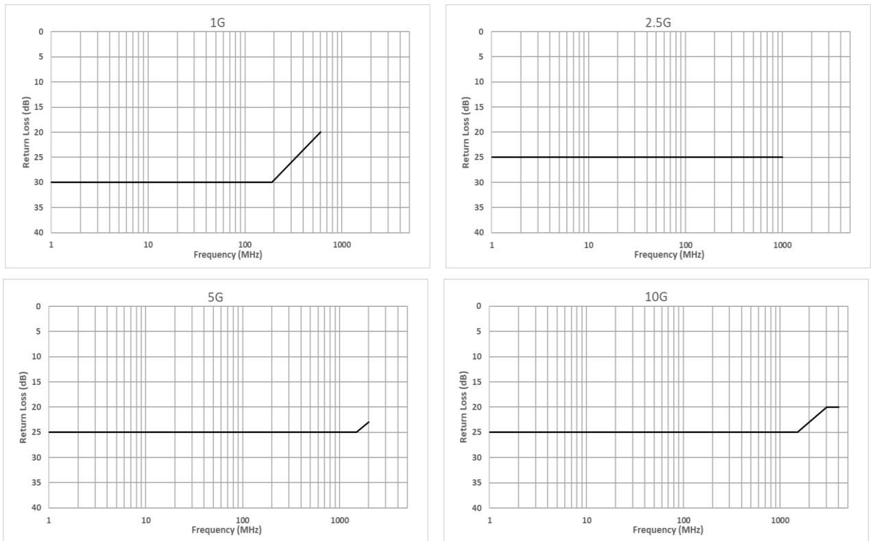
Figure 59: Return loss requirements for mated connector pairs (method A)
