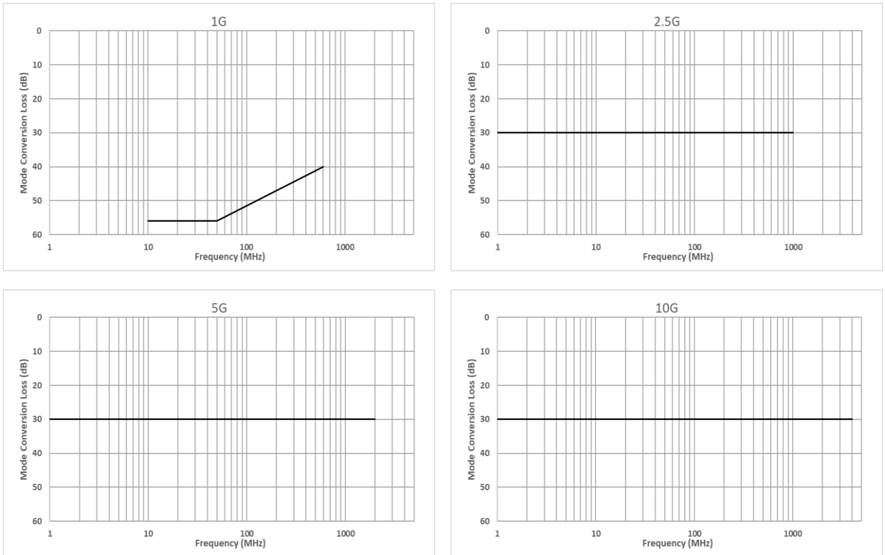
Figure 31: Balance requirements on MDI test heads
