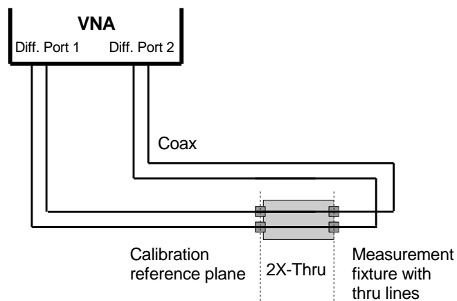
Figure 35: PCB measurement fixture 2X-Thru measurement setup
