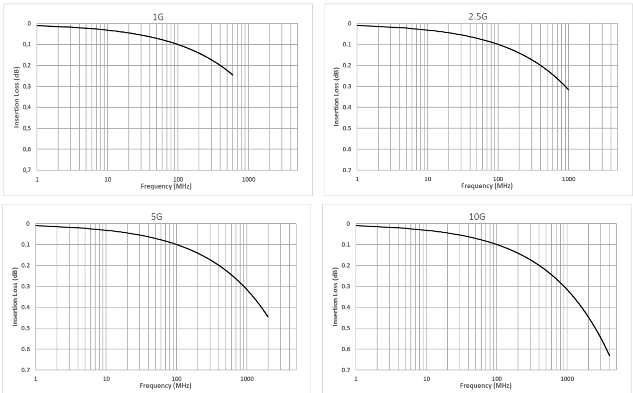
Figure 60: Insertion loss requirements for mated connector pairs (method A)
