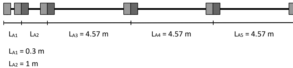
Figure 96: Reference communication channel RCC4, nominal length 15 m
