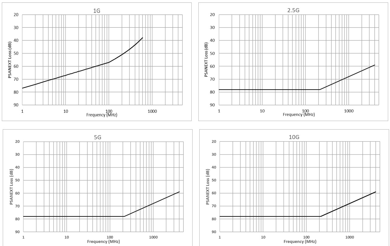
Figure 68: PSANEXT Loss requirements for connectors
