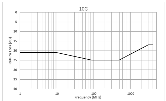
Figure 65: Return loss limit for cable assemblies
