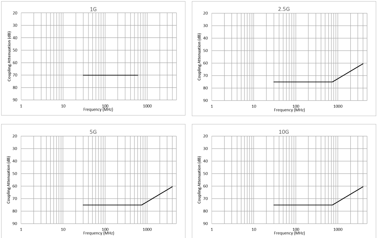
Figure 74: Coupling attenuation requirements for cable assemblies
