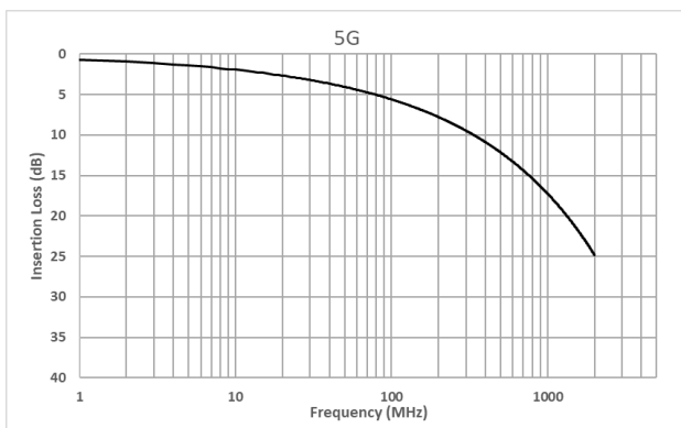
Figure 66: Insertion loss requirements for whole communication channel
