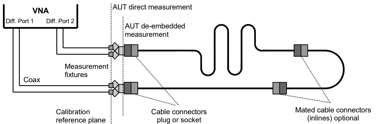
Figure 54: VNA measurement setup for communication channels
