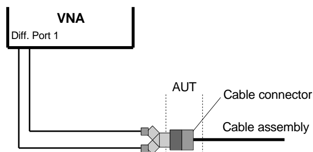
Figure 36: Measurement setup for cable connector return loss measurements
