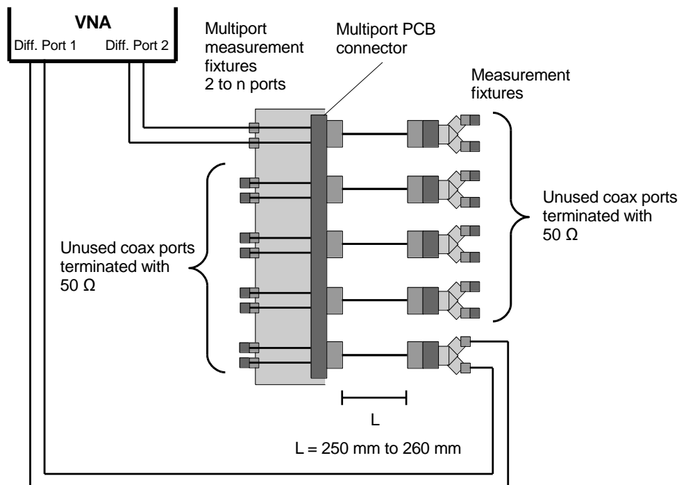
Figure 39: Multiport PCB connector measurement setup for AFEXT Loss
