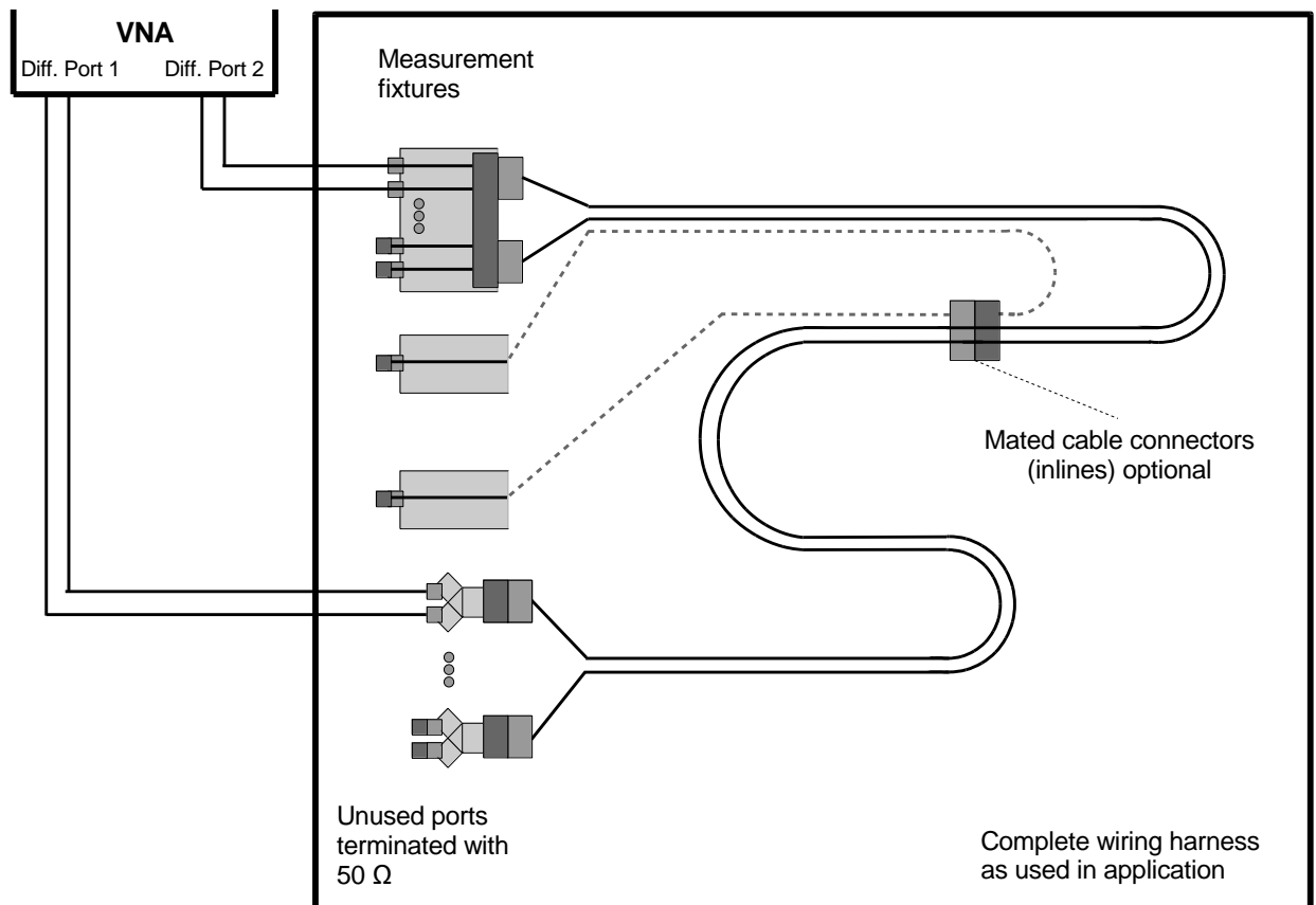
Figure 56: Wiring harness measurement setup for AFEXT Loss and Thru
