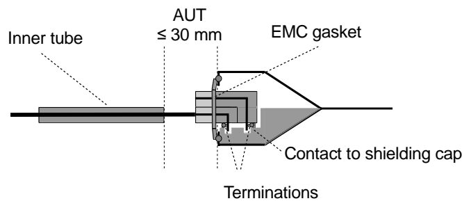
Figure 44: Definition of termination for multipoint connectors with EMC gasket or as cable connector measurement termination
