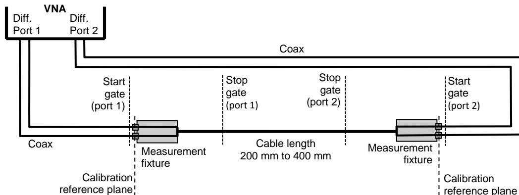
Figure 23: Measurement setup for direct cable measurement fixture characterization
