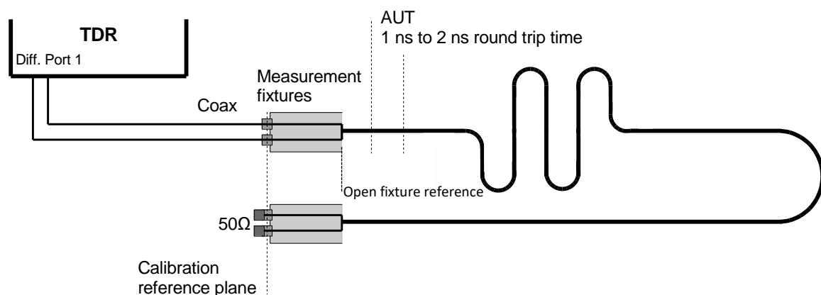
Figure 50: TDR measurement setup for cables
