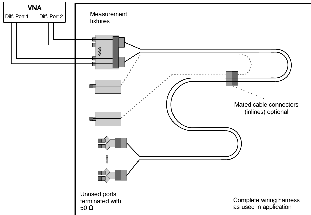
Figure 57: Wiring harness measurement setup for ANEXT Loss
