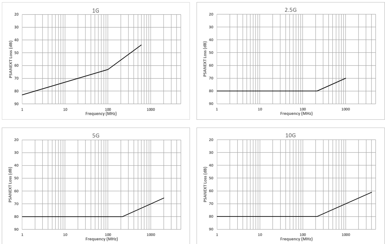
Figure 22: PSANEXT Loss requirements for multipoint measurement fixture cross talk
