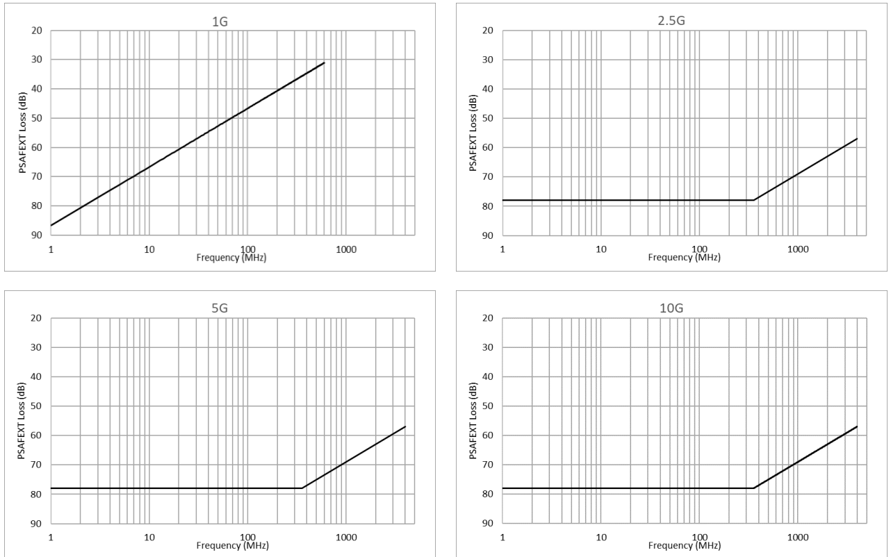
Figure 69: PSAFEXT Loss requirements for connectors
