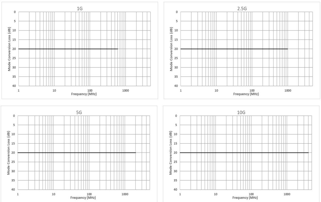
Figure 64:LCTL limit for cables
