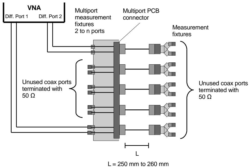
Figure 40: Multiport PCB connector measurement setup for ANEXT Loss
