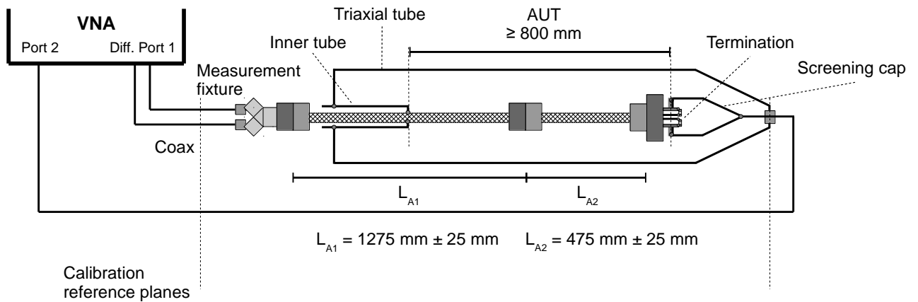
Figure 58: Coupling and screening attenuation reference channel assembly
