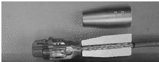
Figure 88: Inline and PCB connector shield contact preparation for coupling and screening attenuation measurement example
