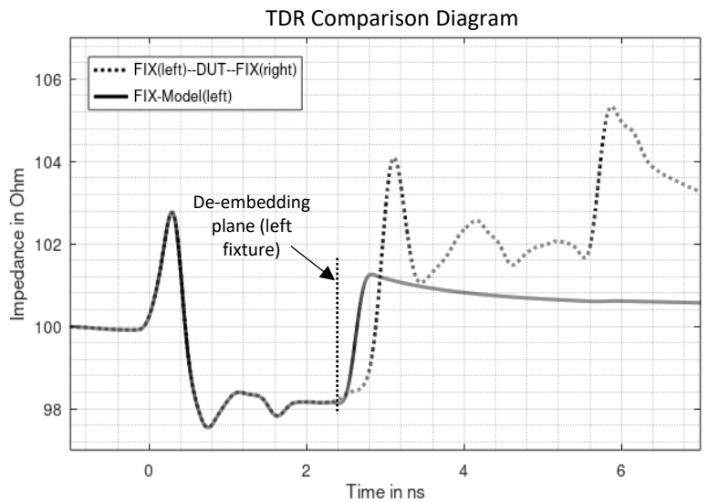
Figure 13: Consistency test #2 - comparison of fixture model and FIX-DUT-FIX structure, example for inline connector de-embedding
